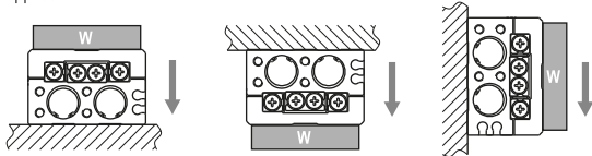
Fig. 1: Applied load
